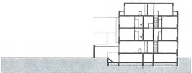
BB' SECTION
